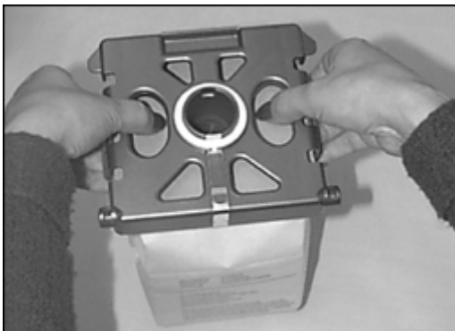
Fig 3. Remove the Filter Bag from the Retainer by pulling out the clips on the side of the retainer and pressing on the cardboard end of the Filter Bag. Take care not to let the Filter Bag drop.
